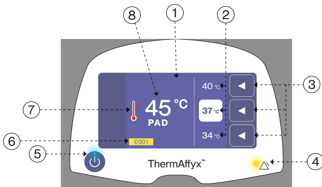
Fig. 5 Control Panel
